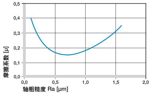
不同的轴表面光洁度下的摩擦系数 (Cf53钢轴) Coefficient of friction as function of the shaft surface (shaft Cf53)
